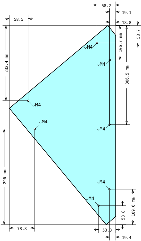
DRAWING 5, Pos 7 Hole placement
