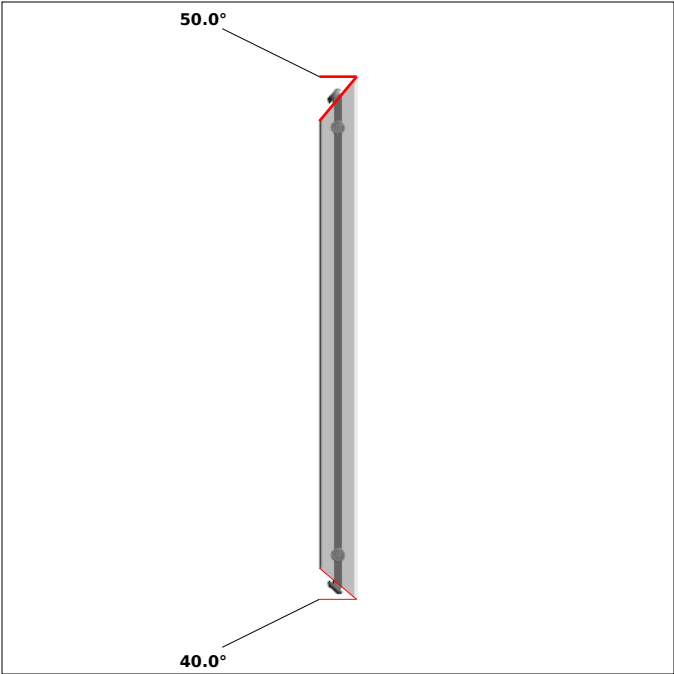
DRAWING 4, Pos 6 SIDE 1, bar length: 560.1 mm
