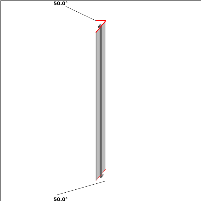
DRAWING 3, Pos 3 SIDE 1, bar length: 638.9 mm
