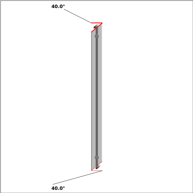
DRAWING 1, Pos 1 SIDE 1, bar length: 529.6 mm
