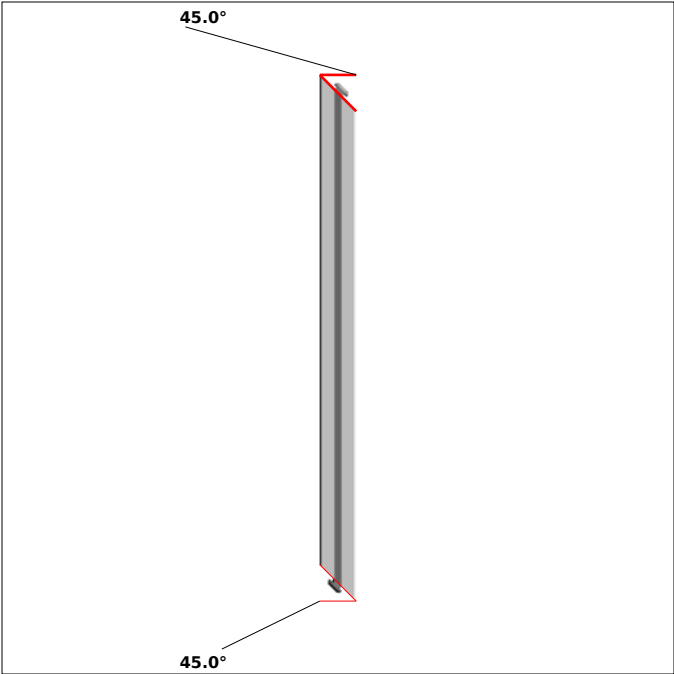
DRAWING 2, Pos 2 SIDE 1, bar length: 577.4 mm
