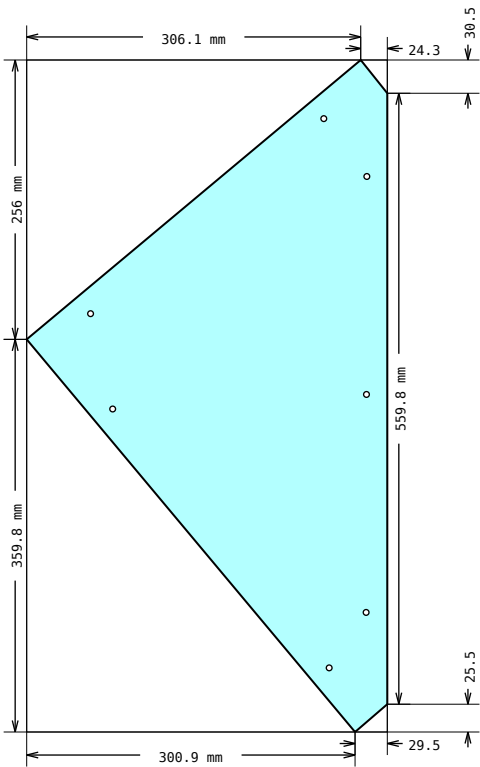
DRAWING 5, Pos 7 Shape measurements
